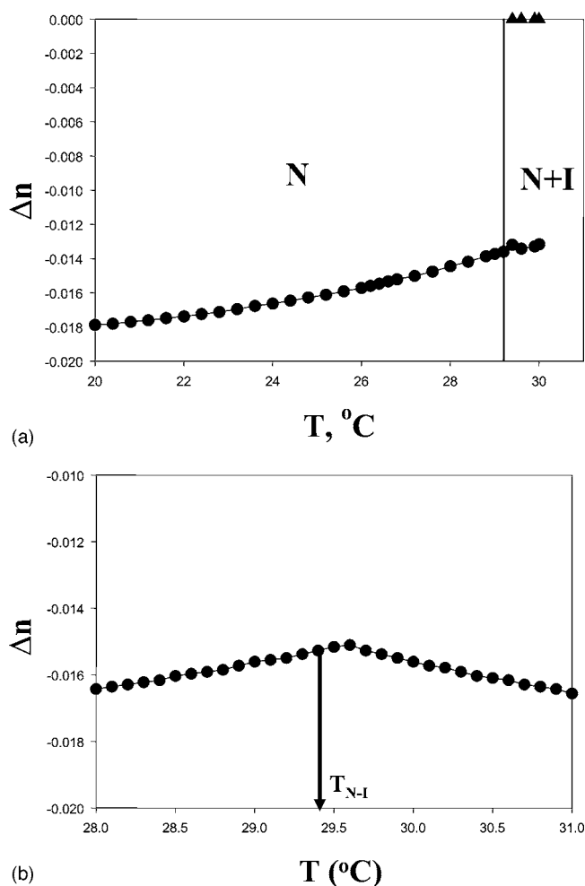
FIG. 10. \Delta n(T) of DSCG, c = 15\text{ wt\%} for two wavelengths \lambda = 633 (a) and 546\text{ nm} (b), respectively. Circles correspond to the N phase, triangles to the I phase. Points above the N - I phase transition were obtained for the nematic and isotropic parts of the biphasic region using a pinhole.
